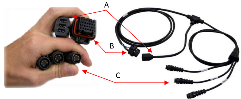
A. John Deere Power Input Plug B. 26-pin Tyco Connector C. 5-pin Female Switchcraft Connectors (Qty 3)
