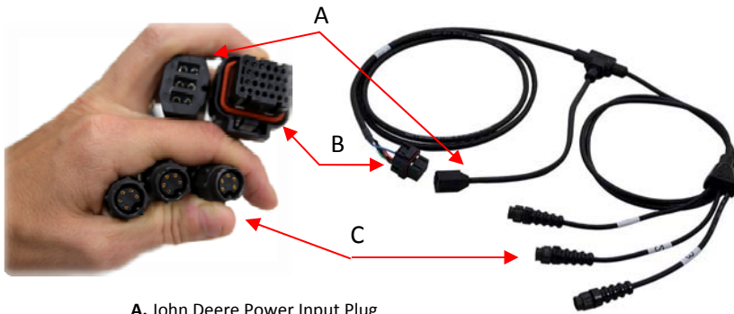
A. John Deere Power Input Plug B. 26-pin Tyco Connector C. 5-pin Female Switchcraft Connectors (Qty 3)
